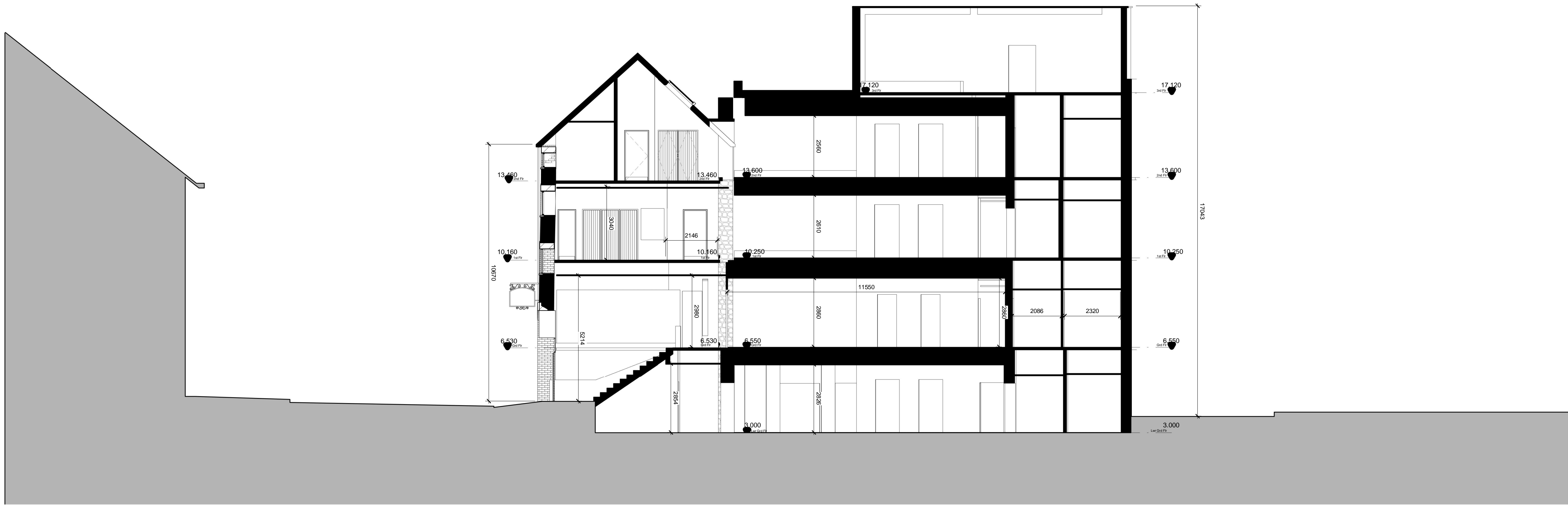
1 Existing Granary Section (South)
